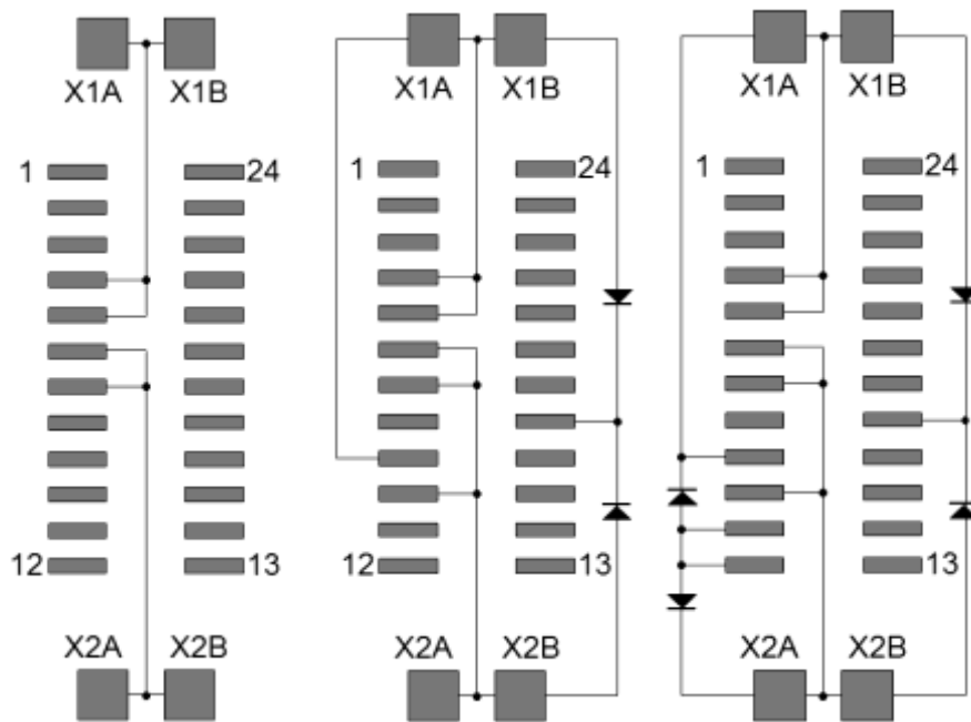
Minimal Jumper Plug
