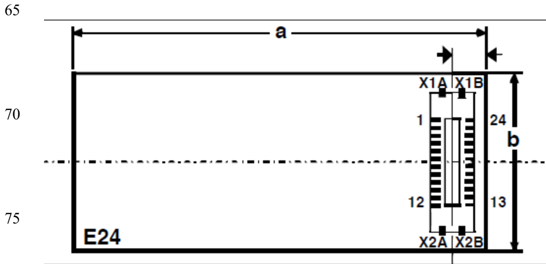
Figure 4: View of the decoder from below, component side of the socket
