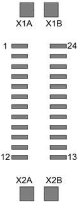
Figure 7: Pin Arrangement for E24 Interface
